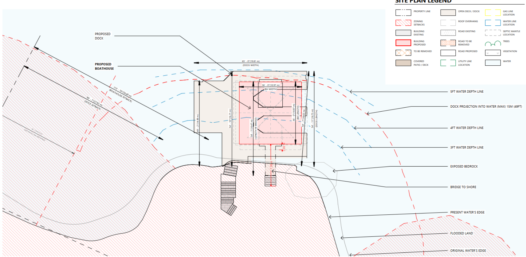
Figure 3: Proposed Boathouse and Dock
